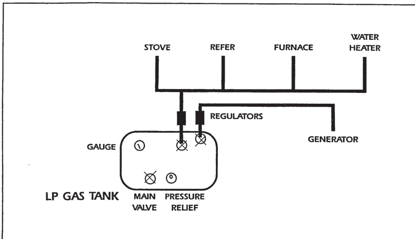
Liquid Petroleum Gas System (Generalized)
